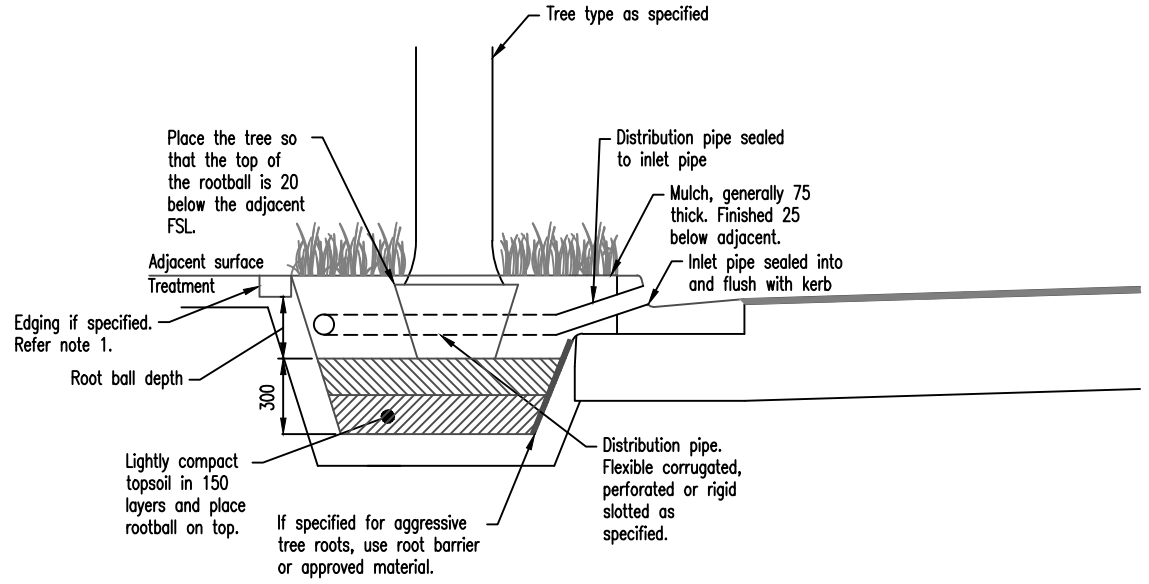
Inlet and kerb detail
