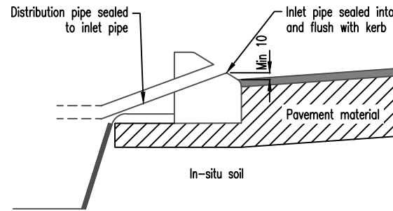
Alternate inlet and kerb detail
