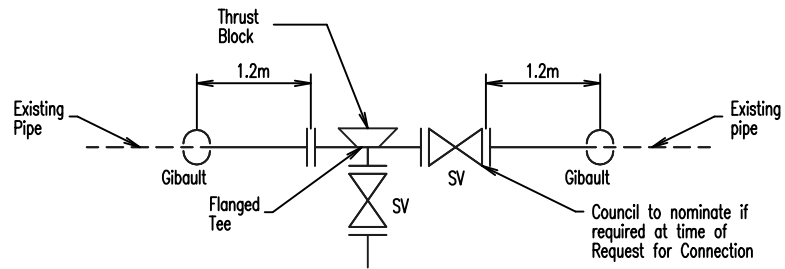
TEE CONNECTION
