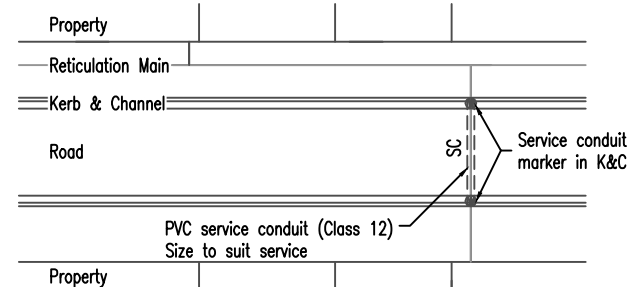
TYPICAL MAIN CONNECTIONS PLAN VIEW
