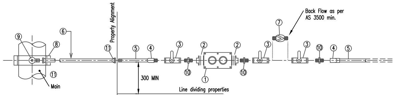
METER SINGLE SERVICE SIDE VIEW
