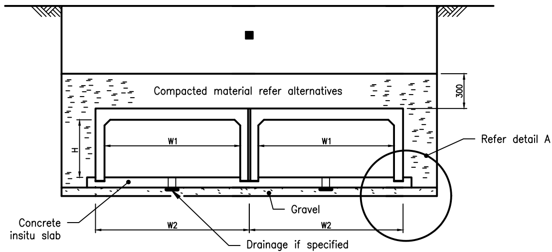
MULTIPLE CULVERTS
