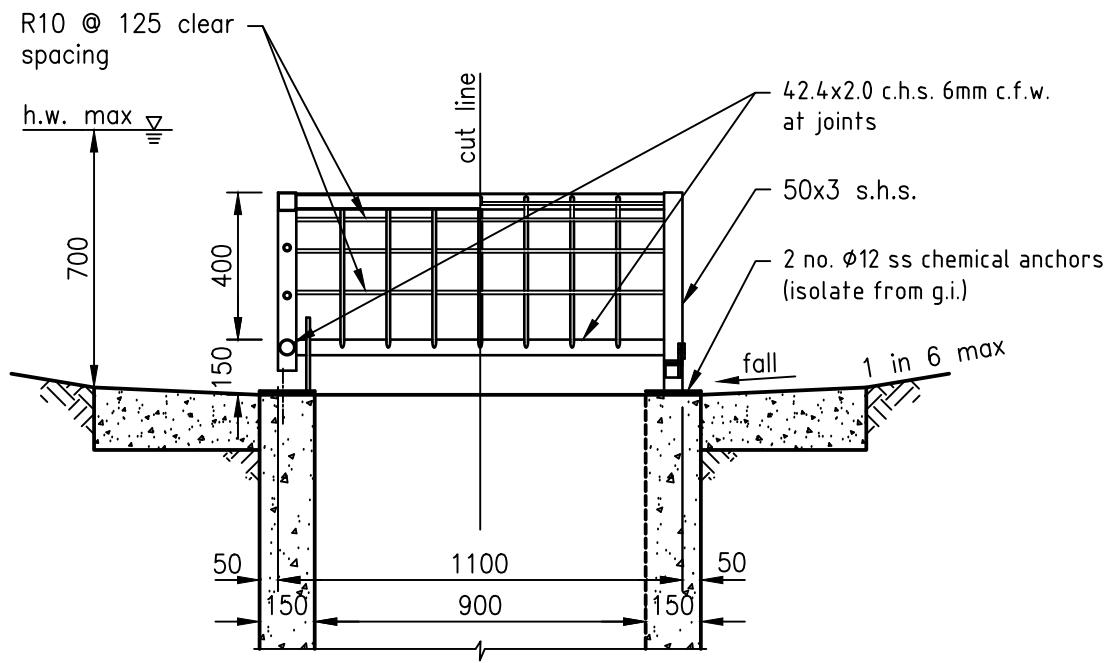
SECTION B-B TYPE 1 GENERAL USE
